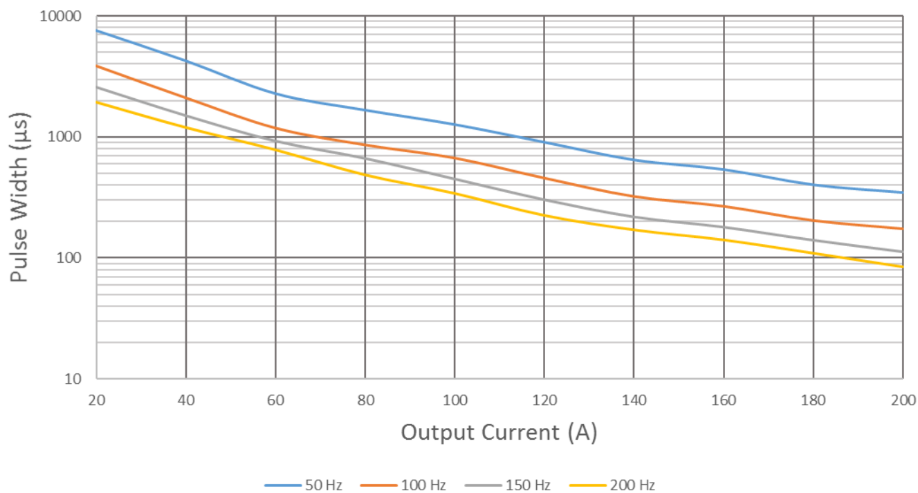
Maximum Pulse Width vs. Output Current
