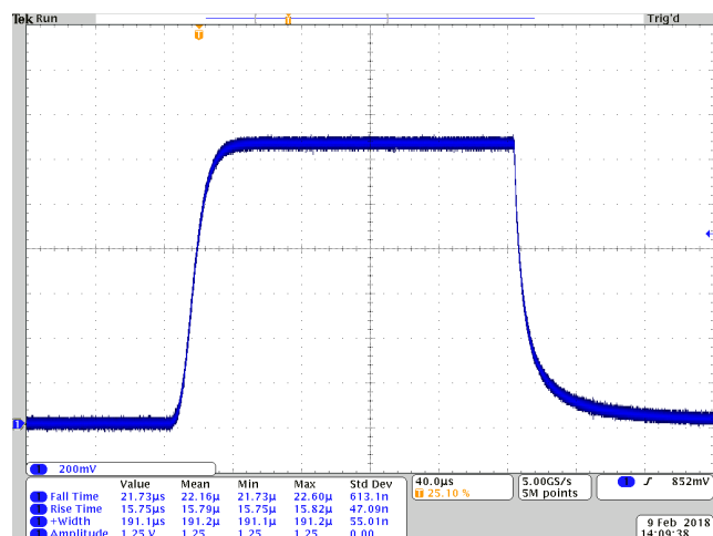
20 A, 200 \mu s pulse width
