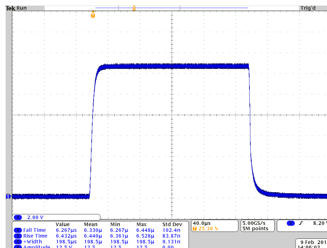
200 A, 200 \mu s pulse width
