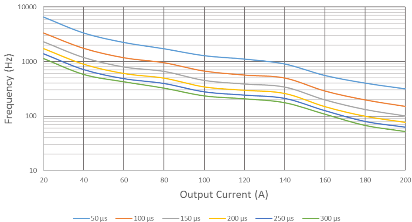
Maximum Frequency vs. Output Current
