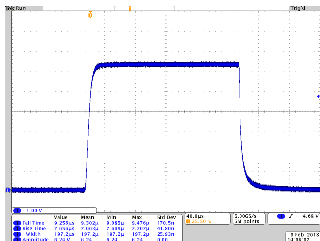
100 A, 200 \mu s pulse width
