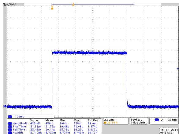
0.5 A, 12.5 V compliance, 20 Hz, 8,750 \mu\text{s} pulse width
