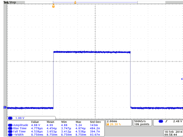
5 A, 17.0 V compliance, 20 Hz, 8,750 \mu\text{s} pulse width
