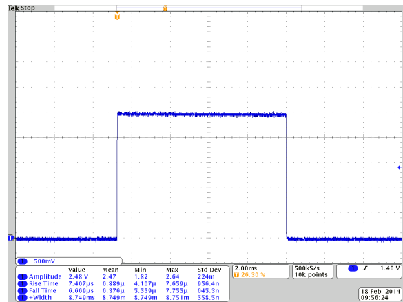
2.5 A, 14.0 V compliance, 20 Hz, 8,750 \mu\text{s} pulse width
