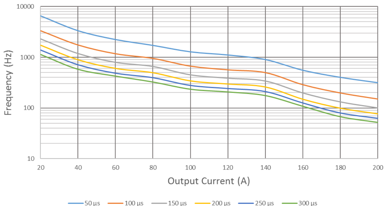
Maximum Frequency vs. Output Current
