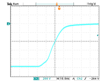
Pulse Fall Time: 25ns at 950V 10ns/Div horizontal scale, 200V/Div vertical scale
