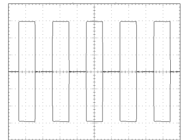
20KHz Frequency, Both Channels 25µs/Div horizontal scale, 318V/Div vertical scale
