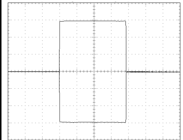
Typical Differential Output, ±950V 2.5µs/Div horizontal scale, 318V/Div vertical scale, center horizontal trace is ground
